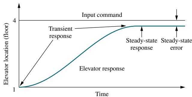
FIGURE 1.2 Elevator response
