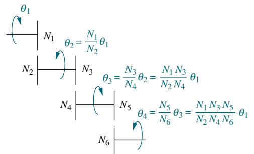
FIGURE 2.31 Gear train
